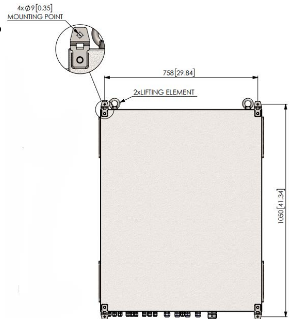
Figure 5-2: RS300 Series Electrical Cabinet Mounting Holes
