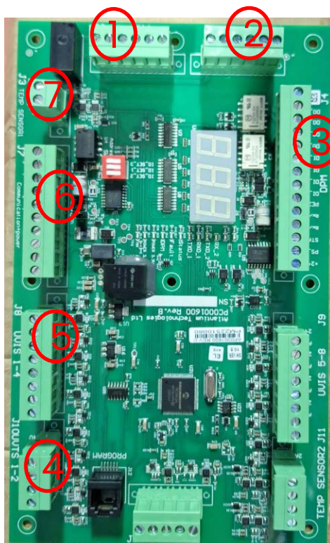
Figure 5-5: Signal Connections on 1600 Connection Card
