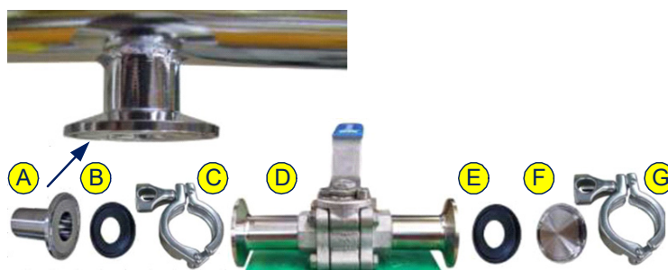
Figure 3-6: CIP Valve Kit
