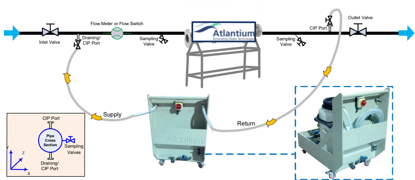
Figure 3-5: CIP Recirculation System Connections
