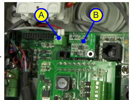
Figure 10-17: Location of the Temperature Sensor Connector (Generic)
