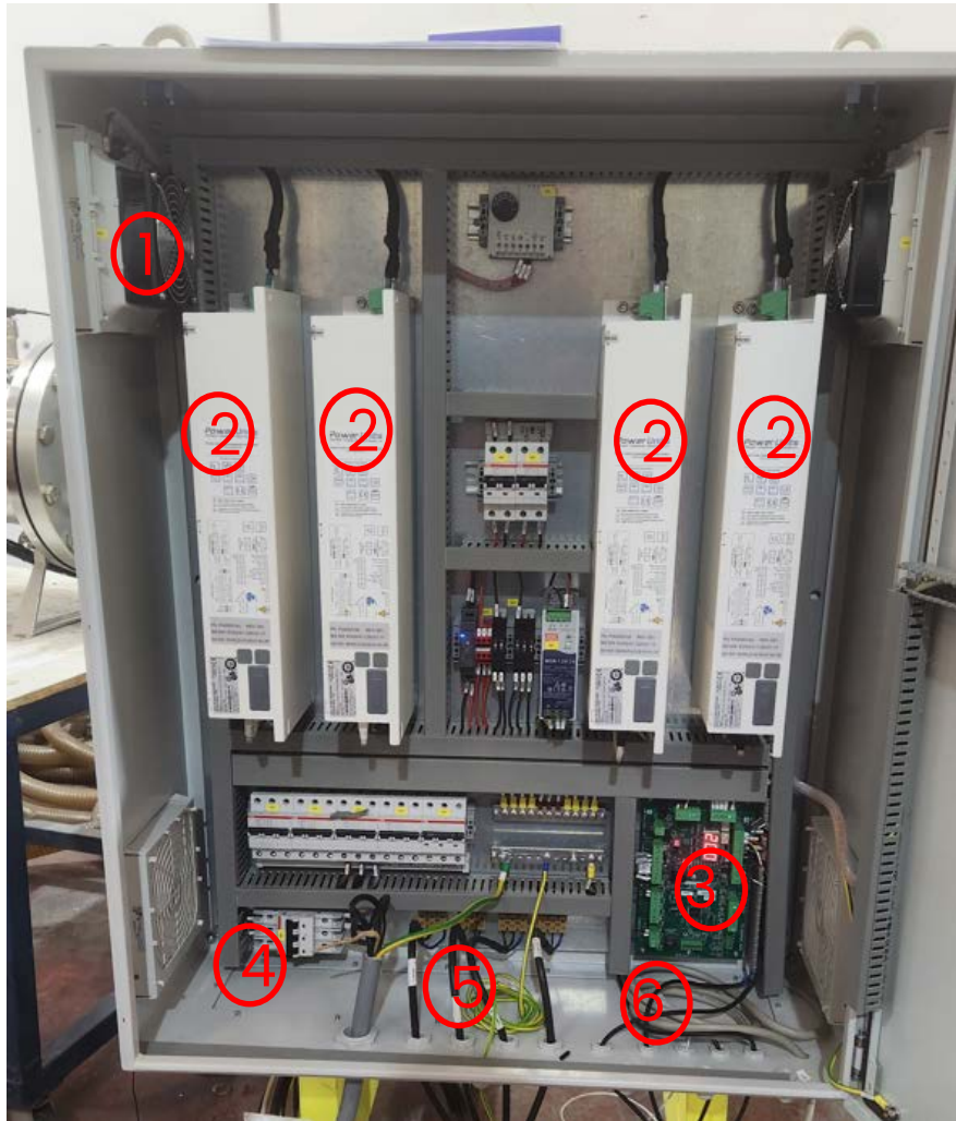
Figure 2-2: RS300 Series Electrical Cabinet -Internal view
