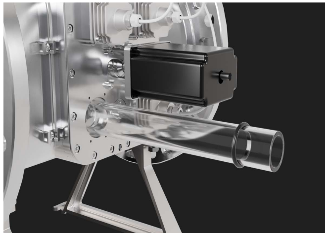
Figure 10-8: Replacing the Quartz Sleeve (Generic View 1)
