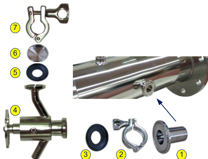
Figure 3-4: Sampling Valve Assembly
