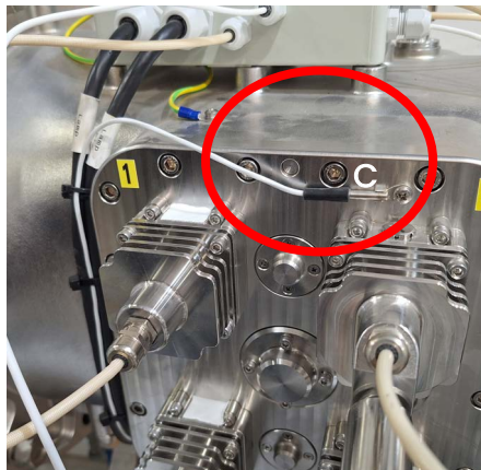
Figure 10-19: Location of the Temperature Sensor
