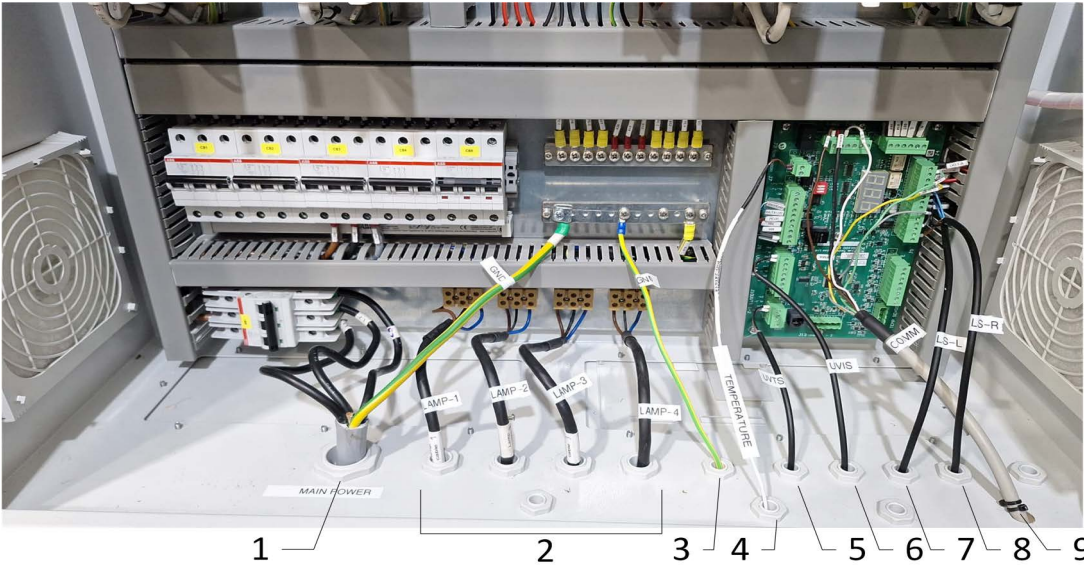
Figure 5-4: Cables Connections in the Electrical Cabinet
