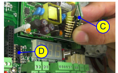
Figure 10-20: Replacing the Temperature Sensor Card (Generic)
